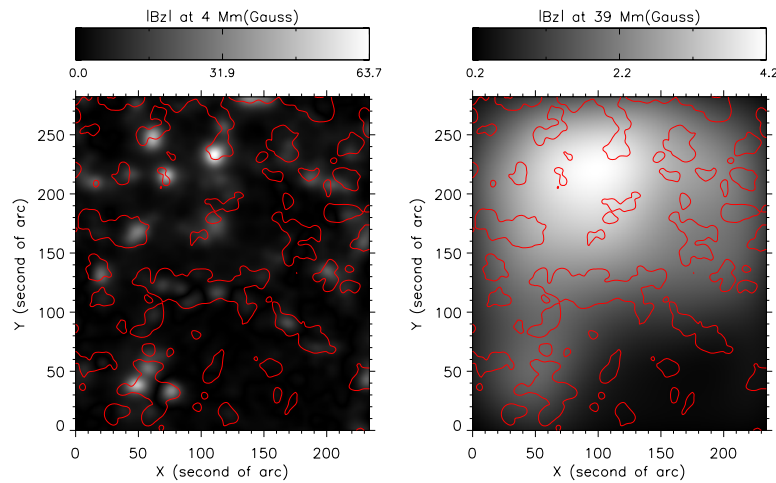
Fig. 5 Extrapolated magnetograms at 4 Mm (left) and 39 Mm (right). The contours taken from Fig. 4 represent bright emission of N IV.
