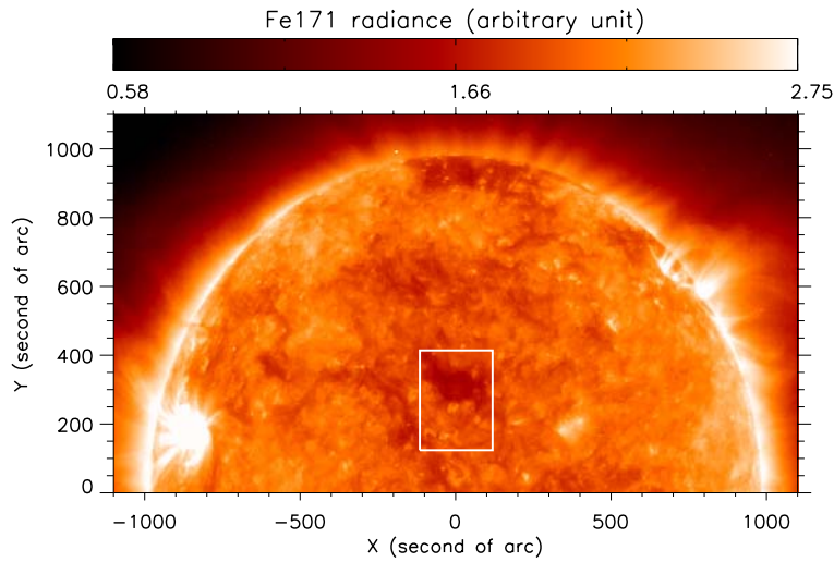
Fig. 1 EIT image (Fe IX/X 171 Å) taken on 1997 March 8, 07:00:13 UT. The area scanned by SUMER/SOHO is outlined by the white rectangle.
