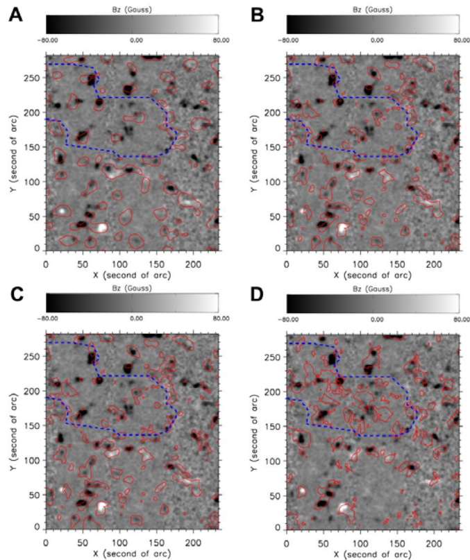
Fig. 4 Magnetogram reconstructed by piecing together 15 slices taken respectively from MDI magnetograms observed at 15 different times during the SUMER raster scan. The thick blue dashed line outlines the boundary of the equatorial coronal hole and the surrounding quiet Sun. The red contours represent bright patches seen on the filtered intensity image (upper) and patches with large shift seen on the dopplergram (lower) for N IV (left) and Ne VIII (right). The contour level of the Doppler shift is 10 \text{ km s}^{-1} (red shift) for N IV, and -5 \text{ km s}^{-1} (blue shift) for Ne VIII.
