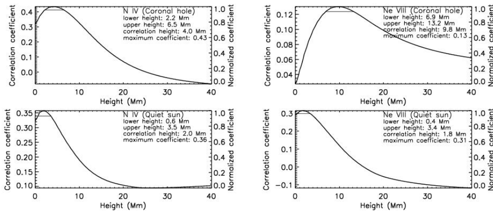
Fig. 6 Height variations of the correlation coefficient between the radiance of N IV and |B_z| (left), and between the blue shift of Ne VIII and |B_z| (right), in the coronal hole (upper) and the quiet Sun (lower). The horizontal bars show the height ranges in which the coefficients are above 95% of the maxima. The y -axis on the right side of each sub-figure indicates the normalized coefficient.
