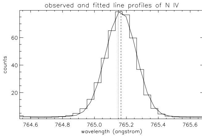
Fig. 2 Observed (histogram) and fitted (smooth line) line profiles of N IV. The dotted and dashed vertical lines indicate the positions of the rest wavelength and the center of the fitted profile, respectively.
