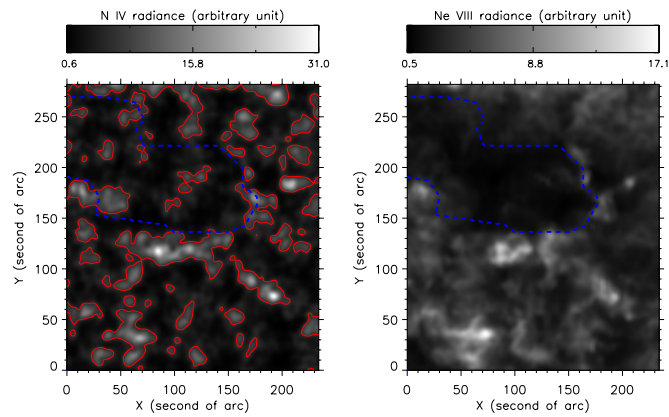
Fig. 3 Intensity images of N IV (left) and Ne VIII (right) in linear scale. The boundary of the coronal hole, indicated by the blue dashed line, was determined by hand and is almost the same as that used in Aiouaz et al. (2005). The contours in the left panel represent patches with large N IV intensity (larger than 6).
