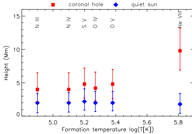
Fig. 7 Temperature variations of the correlation heights in both the quiet Sun and the coronal hole. Squares and diamonds represent the correlation heights and bars indicate the height ranges of emissions.
