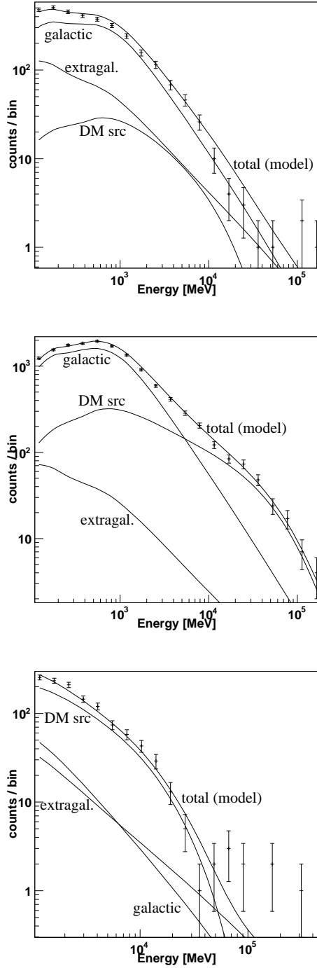
Fig. 4 Examples of spectral fits of simulated DM point sources of intensity \Phi , for different values of m_\chi and different annihilation channels. On the top for \Phi = 2 \times 10^{-3} \text{ ph m}^{-2} \text{ s}^{-1} , m_\chi = 150 \text{ GeV} , b\bar{b} , (l, b)=(0, 25) ; in the middle for \Phi = 2 \times 10^{-2} \text{ ph m}^{-2} \text{ s}^{-1} , m_\chi = 150 \text{ GeV} , b\bar{b} , (l, b)=(50, 0) and on the bottom for \Phi = 2 \times 10^{-2} \text{ ph m}^{-2} \text{ s}^{-1} , m_\chi = 150 \text{ GeV} , 80% b\bar{b} , 20% e^+e^- , (l, b)=(0, 50) . Solid lines are fits obtained under the assumption of annihilation to b\bar{b} . For each model we also give the significance of the detection. Points with error bars are photon counts from the simulated observation.
