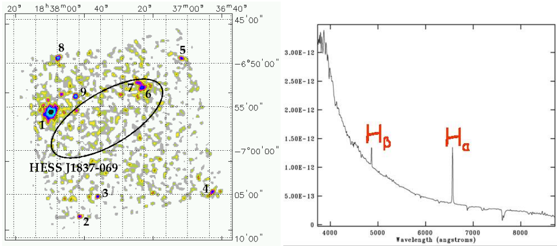
Fig. 6 Left panel : XRT 0.3–10 keV image of the region surrounding HESS J1837–069. The ellipse (with axes of size 14′ and 6′) represents the extension of the TeV source. For details see Landi et al. (2006). Right panel : optical spectrum of the emission-line star HD 259440 acquired in Loiano on April 2007. Balmer H_\alpha and H_\beta emissions, superimposed on a very blue continuum, are apparent. On the y -axis, the fluxes are expressed in \text{erg cm}^{-2} \text{s}^{-1} \text{\AA}^{-1} .
