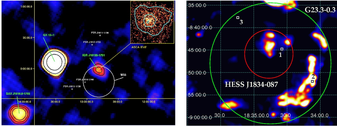
Fig. 5 Left panel : IBIS/ISGRI 20–40 keV image showing the location of HESS J1813–178 and its surroundings. The extension of the TeV source is contained within the contour of the INTEGRAL source IGR J18135–1751. Also shown are the location of SNR W33 (G12.82–0.02) and of the 4 nearest radio pulsars. The extension (15′ radius) of W33 is also indicated by the white circle. The ASCA image at the HESS position is shown as an inset on the top right side of the figure; the box covers an 8′×8′ region centered on the ASCA source position. Coordinates are displayed in the Galactic system. For details see Ubertini et al. (2005). Right panel : radio image at 20 cm of the region surrounding HESS J1834–087. The larger circle (green, 13′ radius) describes the position and extension of SNR G23.3–0.3 as given in Green (2004). The smaller circle (red, 3′ radius) represents instead the extension of the TeV source. The positions of the XRT sources are given by boxes. For details see Landi et al. (2006).
