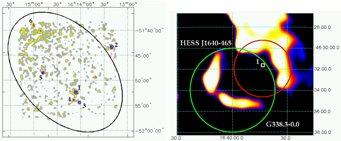
Fig. 4 Left panel : XRT 0.3–10 keV image of the region surrounding HESS J1614–518. The ellipse (with axes of size 28' and 18' ) represents the extension of the TeV source. For details see Landi et al. (2006, 2007a). Right panel : radio image at 843 MHz of the region surrounding HESS J1640–465. The larger circle (green, 4' radius) describes the position and extension of SNR G338.3–0.0 as given in Green (2004). The smaller circle (red, 2\frac{1}{2}' radius) represents instead the extension of the TeV source. The position of the XRT Source 1 is given by a box. For details see Landi et al. (2006).
