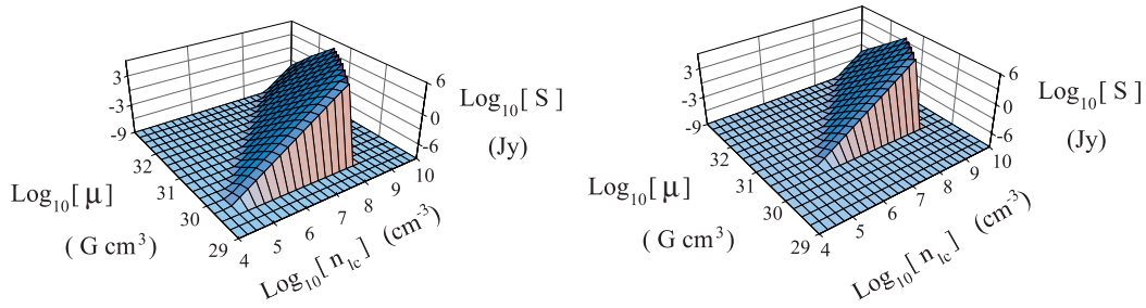
Fig. 4 Predicted angle-averaged flux densities for electron-cyclotron masers, at 5 GHz (left) and 22 GHz (right), from a UI UCD for various loss-cone electron number densities n_{lc} and white-dwarf magnetic moments \mu (Willes, Wu & Kuncic 2004). The orbital period is assumed to be 300 s and the distance, 100 pc. The thermal background electron number density is assumed to be 10^8 \text{ cm}^{-3} and have a temperature of 1 eV.
