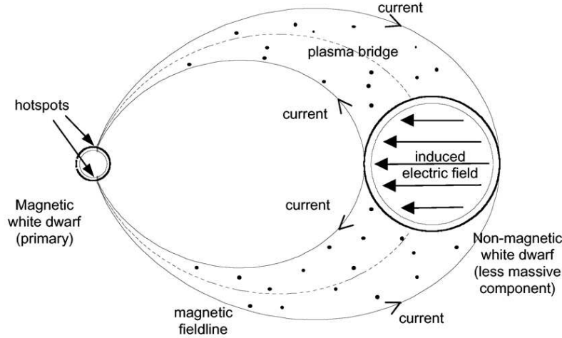
Fig. 1 A schematic illustration of the operation of unipolar induction in a UCD from Wu et al. (2002).
