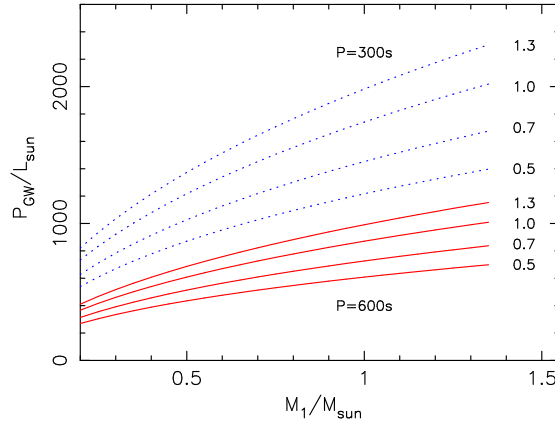
Fig. 3 The power of gravitational waves emitted from UCD as a function of the magnetic white-dwarf mass M_1 , for orbital periods of 600 s (solid lines) and 300 s (dotted lines). Each line corresponds to a value of the companion white-dwarf mass, labeled in solar-mass unit. The gravitational radiation power is normalised to the solar bolometric luminosity.
