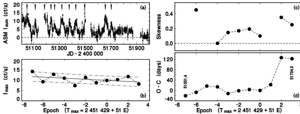
Fig. 3 Evolution of the echo outbursts in KS 1731–260. (a) A part of the ASM/RXTE light curve fitted by HEC13 (smooth solid line). (b) Variations of I_{\text{max}} and their linear fit. (c) Skewness of the outburst light curve. (d) O–C diagram for T_C of the echo outbursts. Only the clearly defined outbursts with the maximum of the fitted curve I_{\text{sum}} > 7\text{ ct s}^{-1} were considered.
