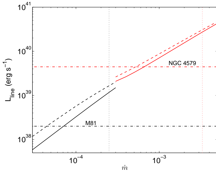
Fig. 2 The total H-like and He-like iron line luminosities as functions of accretion rate \dot{m} calculated for the Honma (1996)'s model. The solid lines correspond to the cases with the solar metallicity, while the dashed lines are for the cases with five times solar metallicity. The observed values for these two sources are marked in the figure (dash-dotted lines). The dotted lines represent the accretion rates derived from the ADAF+SD model fitting on the observed SEDs.
